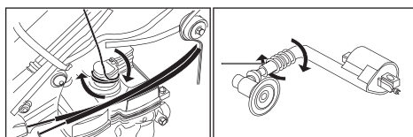
4 stroke installation, wrap pickup wire around head of coil. 2 stroke installation, wrap pickup wire around spark plug lead.
