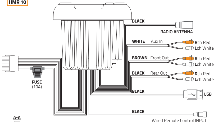
12 PIN HARNESS
