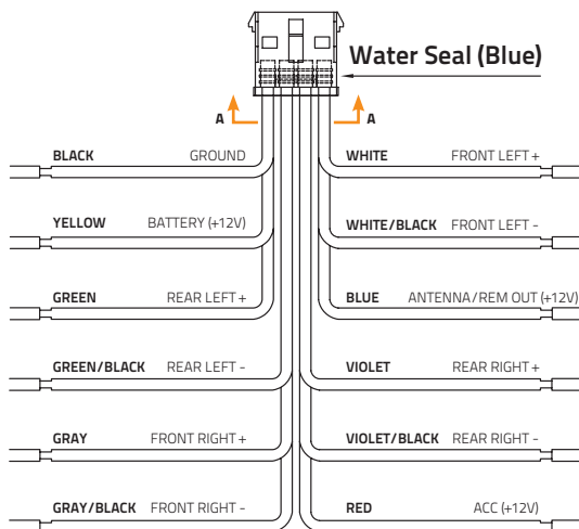
12 PIN HARNESS
