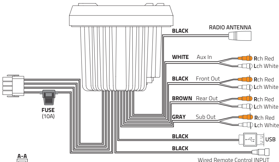
12 PIN HARNESS
